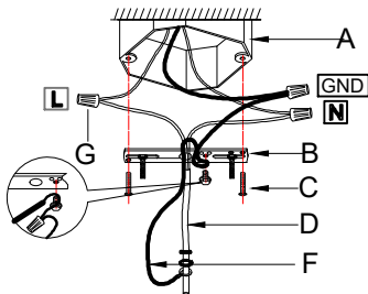
Wire Connection Diagram:
