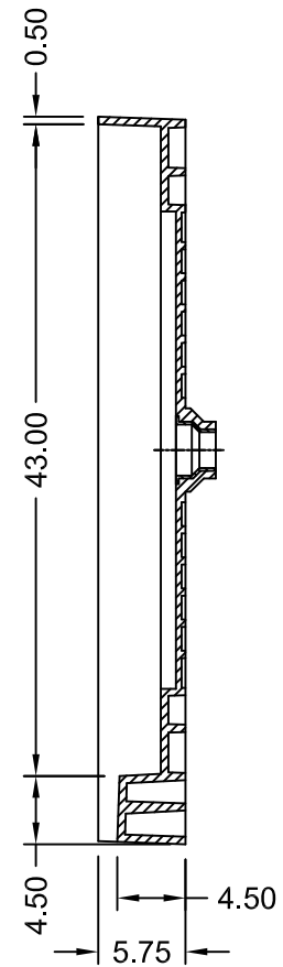
SECTION B-B
