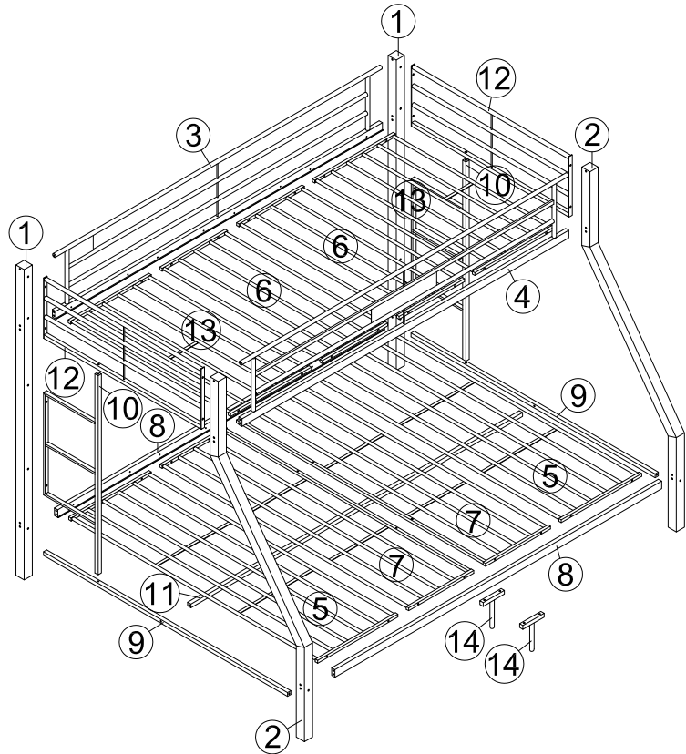
Exploded View
