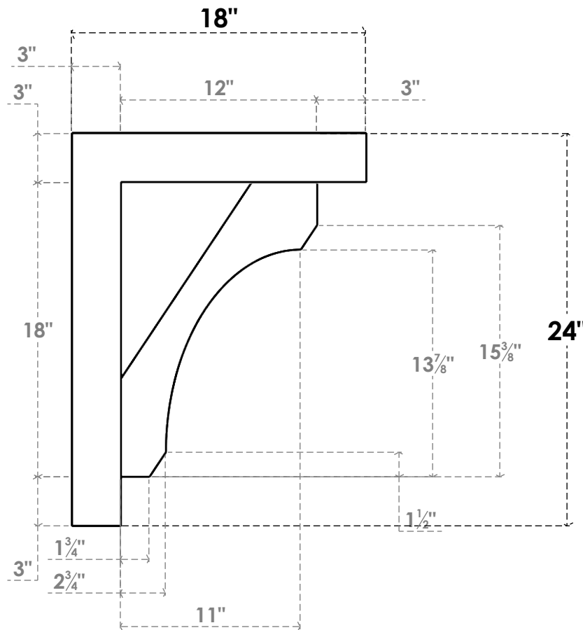
SIDE PROFILE
