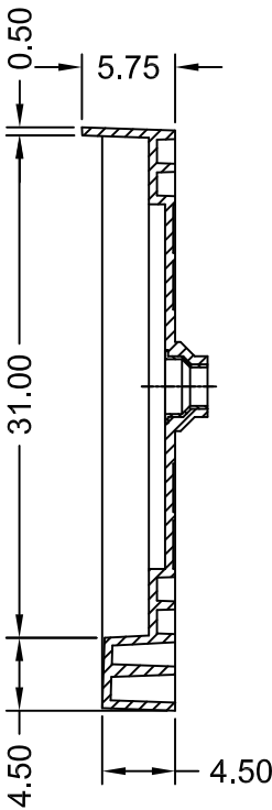
SECTION B-B
