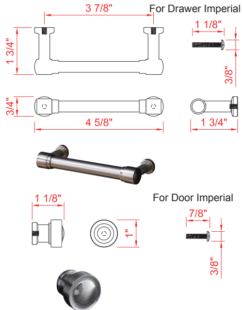
HANDLE
