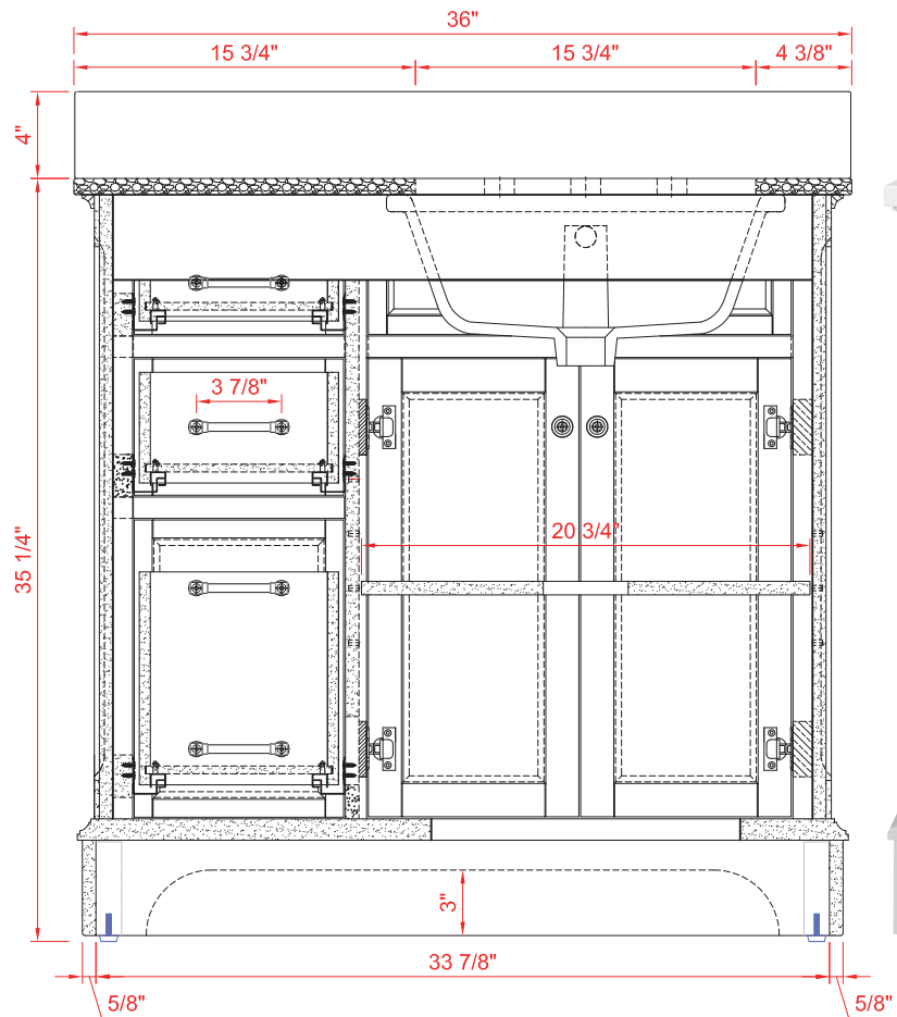
BACK VIEW
