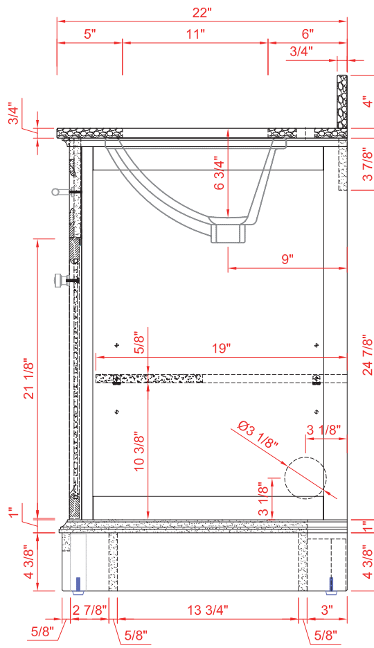
SIDE VIEW
