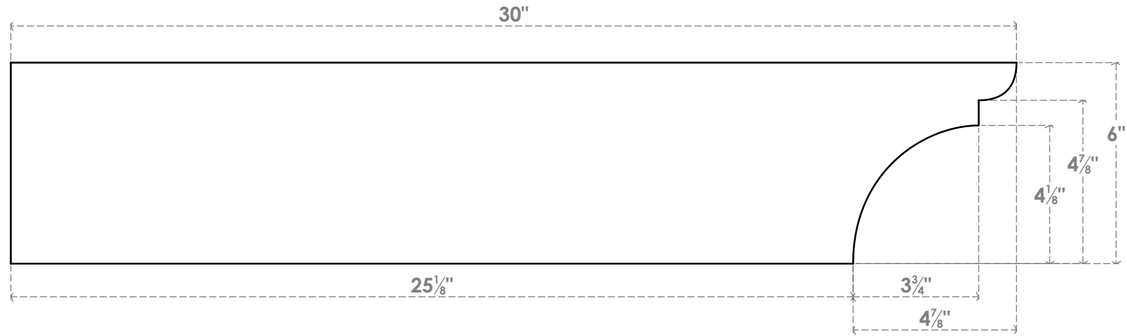
SIDE PROFILE
