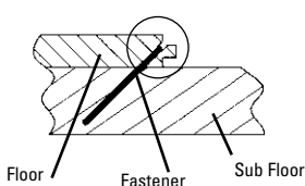
PROPERLY DRIVEN FASTENER
