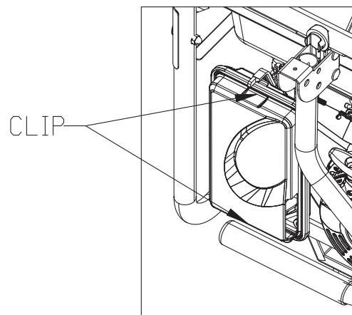
Figure 14 - Air Filter
