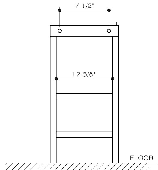
BACK VIEW
