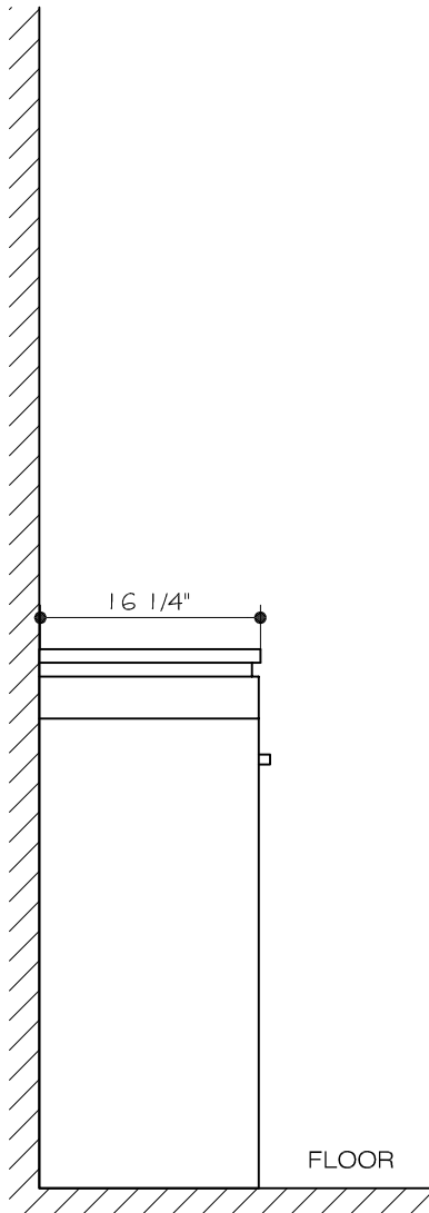
SIDE VIEW
