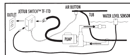
OPTIONAL: MOUNTAIN AIR SWITCH
