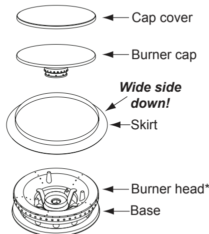
SimmerSear Burner Assembly
