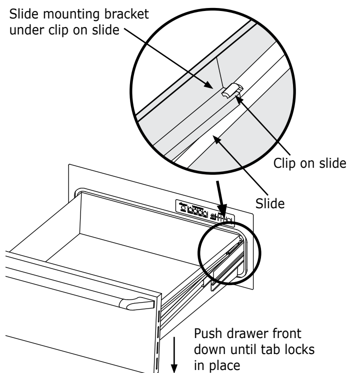
Drawer Installation
