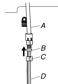
A. Plastic water tubing C. Compression nut B. Sleeve D. Copper tubing
